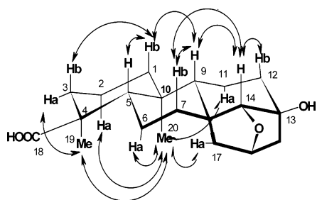
FIGURE 6. Selected NOE interactions of 1 .
